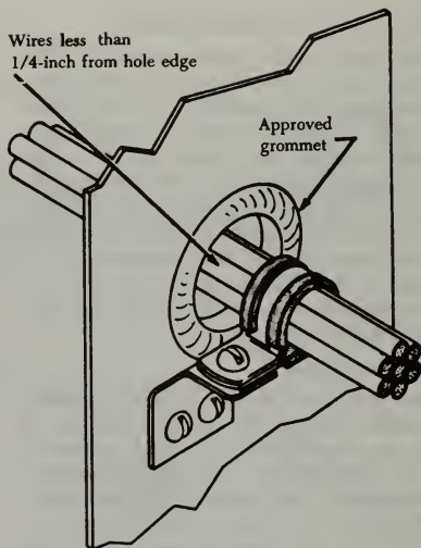
FIGURE 4-93. Cable clamp and grommet at bulkhead hole.
